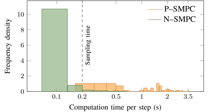
(c) Density histogram for computation times. The N-SMPC computation times for steps that the NLP was infeasible are not considered and the data only account for the duration of sampling times where the planner converged to a solution.
