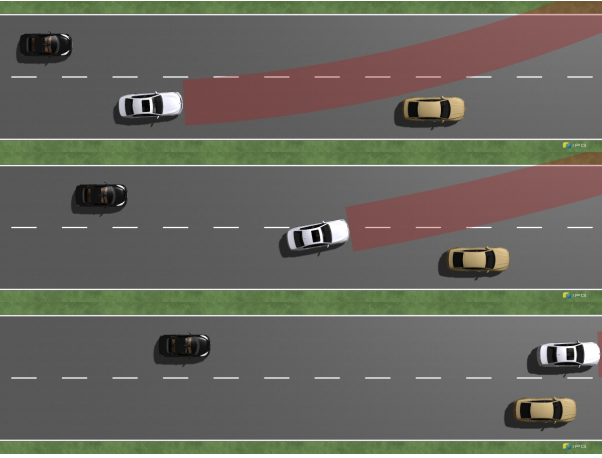
(b) Proactive collision avoidance by P-SMPC: the ego vehicle manages to get out of the risky zone before its front vehicle stops.
