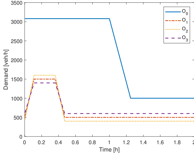
Figure 4: Traffic demand profiles for the origins of the freeway network
