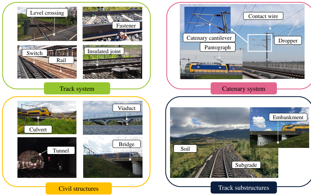
Figure 1. Illustration of the four selected groups of railway infrastructures considered in this work: track system, catenary system, civil structures, and track substructures.
