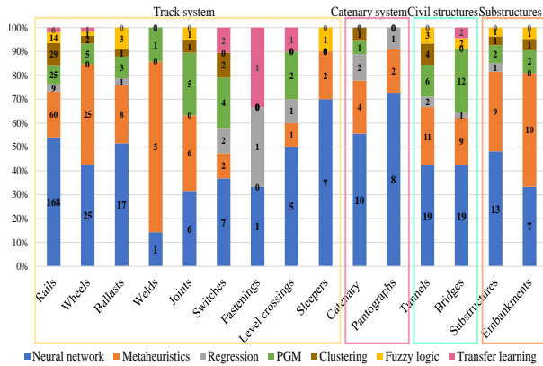
Figure 7. Development of the selected AI methodologies in 2023.
