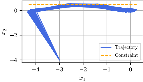
Fig. 1. The closed-loop trajectories, tested on 500 samples, converge to a neighborhood of the origin.
