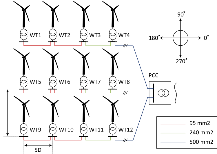
Figure 4: Wind farm layout.
