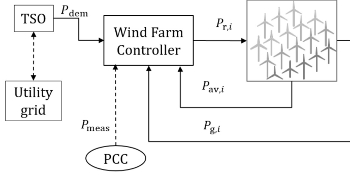
Figure 2: Closed-loop control scheme.
