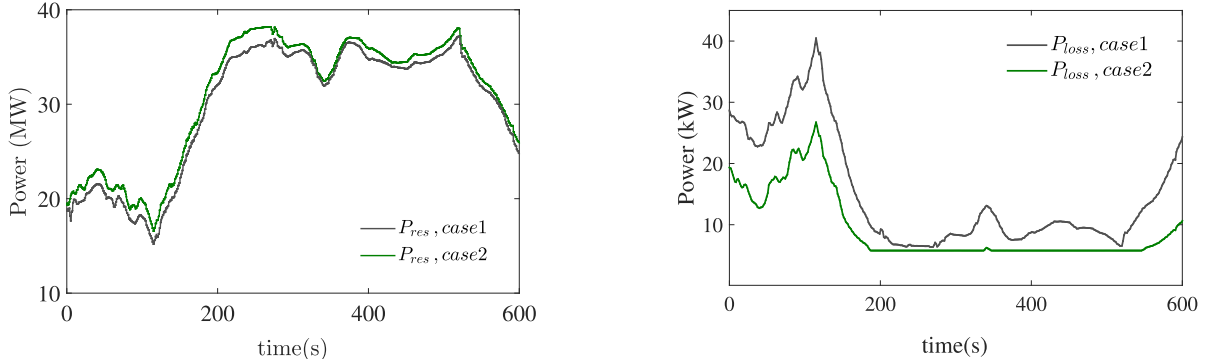
Figure 7: Scenario 1: Power reserve and power losses profiles.
