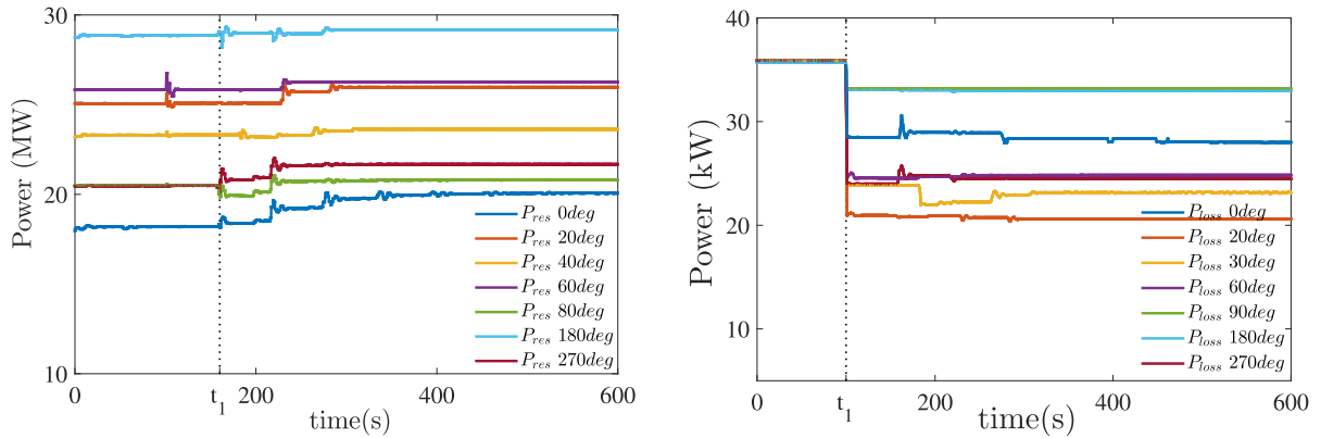
Figure 9: Power reserve and power loss for several wind direction.
