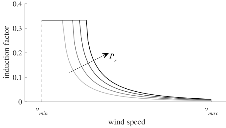
Figure 3: Induction factor a - wind speed v characteristic for several power set-points P_r .
