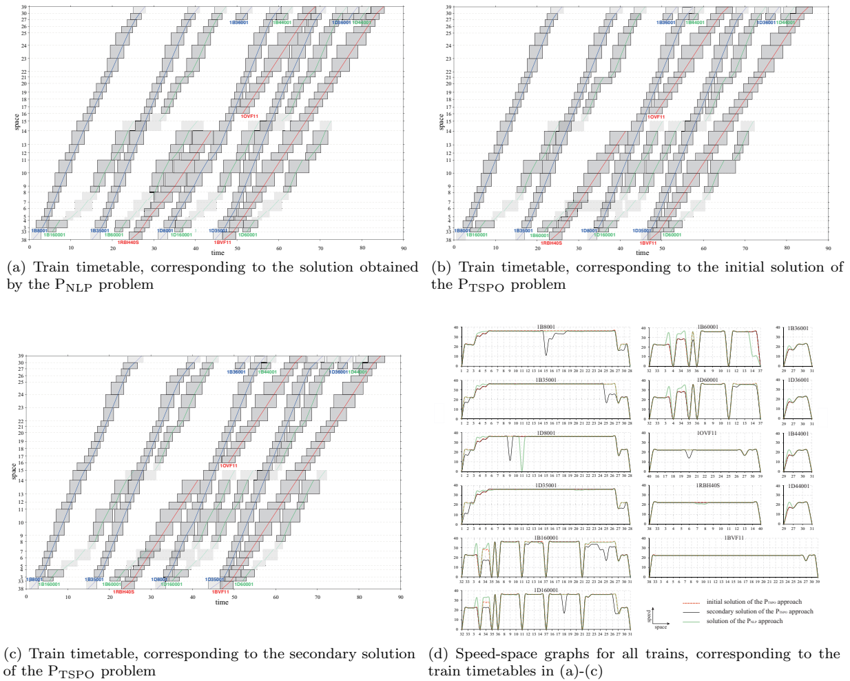
Fig. 14. Train timetables and train speed-space graphs for the Dutch railway network
