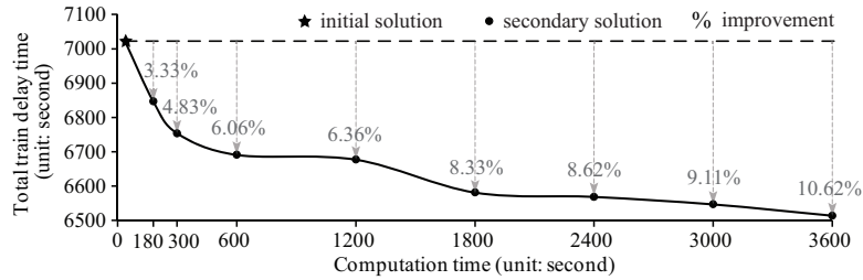
Fig. 16. Total train delay time as a function of computation time, results for the INFORMS RAS railway network
