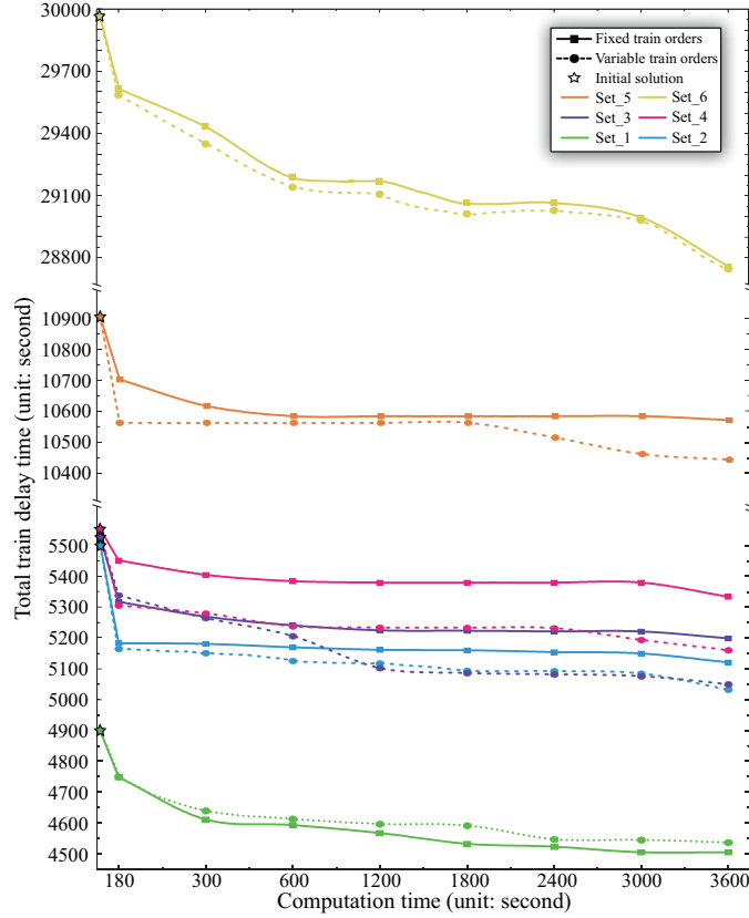
Fig. 10. Total train delay time of the 6 sets as a function of computation time
