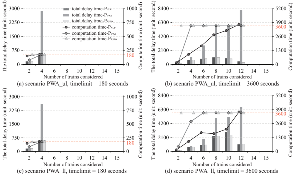
Fig. 6. Results of the three optimization approaches, corresponding to the feasible cases of the P_{PWA} approach
