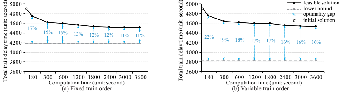
Fig. 12. Lower bounds, feasible solutions, and estimation of optimality gaps
