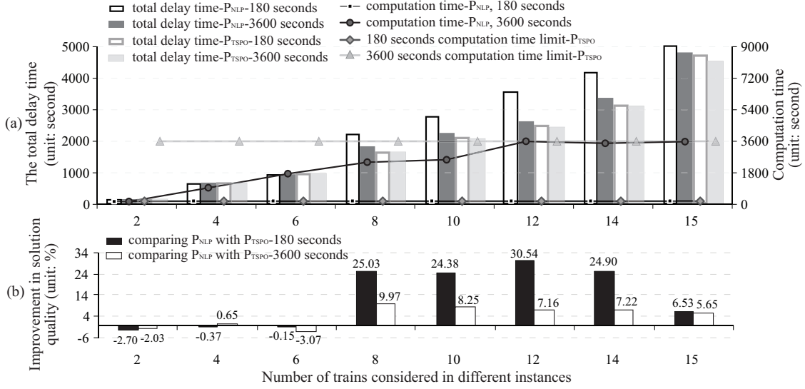
Fig. 7. Results of the P_{NLP} problem and the P_{TSPO} problem
