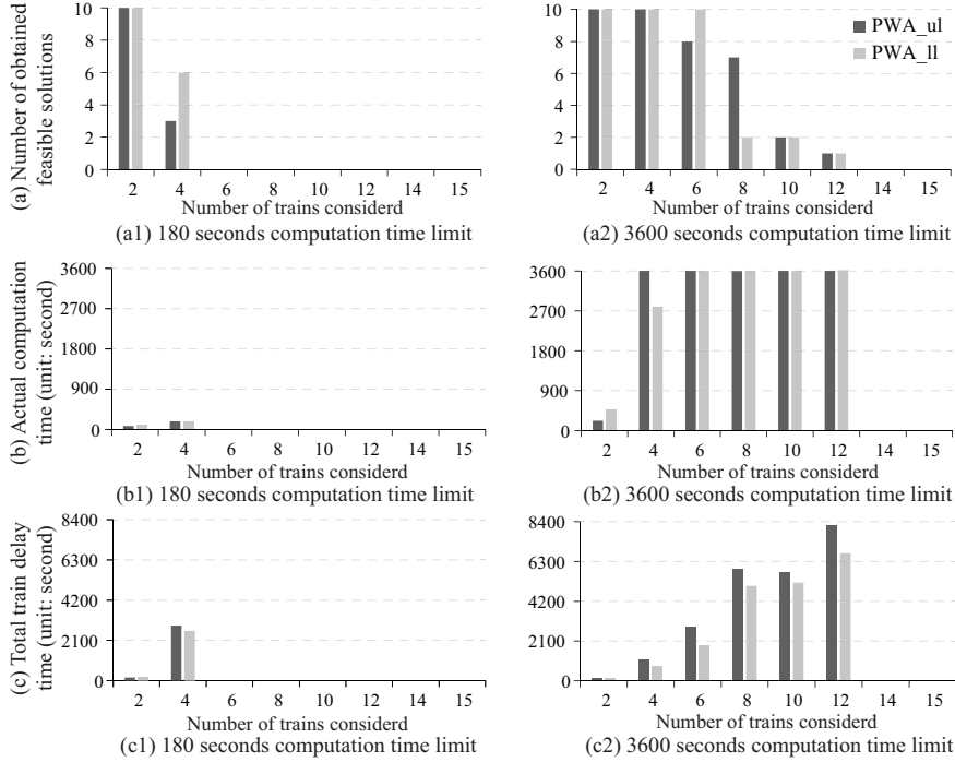
Fig. 8. Results of the P_{PWA} problem, for “PWA_ul” and “PWA_ll”
