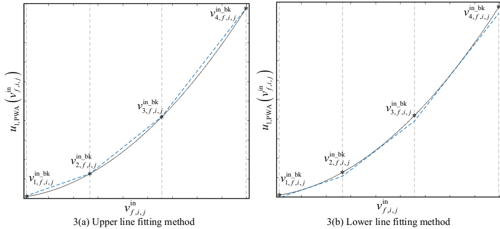
Fig. 3. The PWA approximation of the non-linear function
