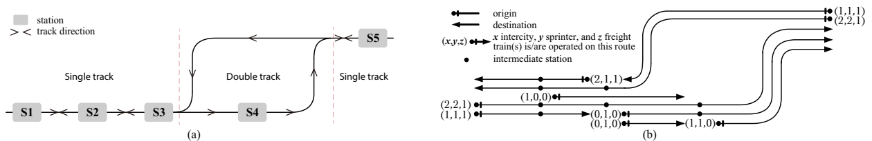
Fig. 15. A rail network adapted from INFORMS RAS (2012)
