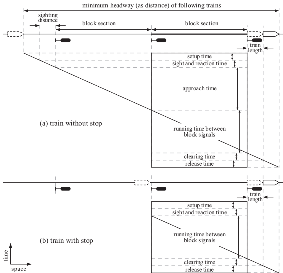
Fig. 1. The blocking time of a block section for a train without/with a scheduled stop
