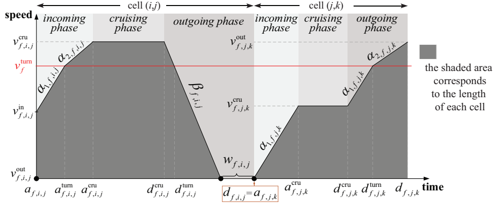
Fig. 2. Speed-time graph of train f on cell (i,j) and cell (j,k) to illustrate the relevant decision variables
