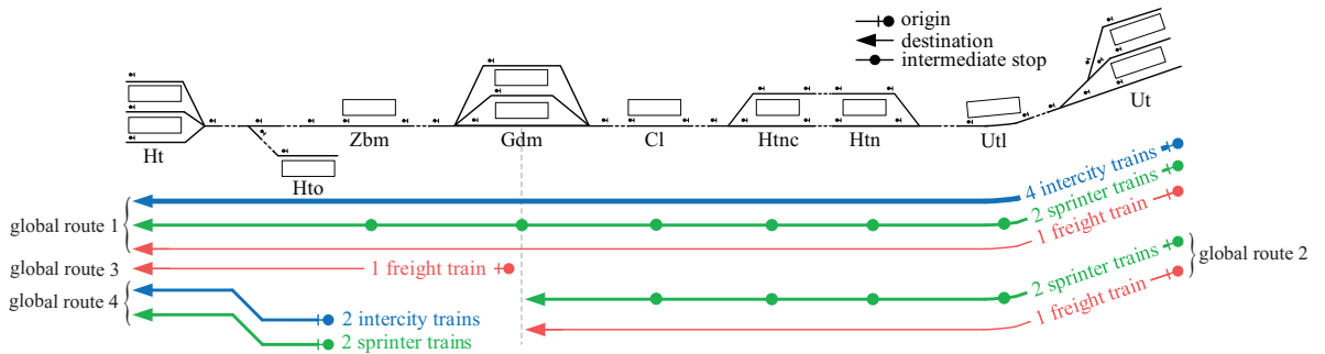
Fig. 5. A real-world experimental network adapted from the Dutch railway network
