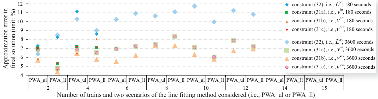
Fig. 9. Approximation errors of the constraints in the P_{PWA} problem, for “PWA_ul” and “PWA_ll”
