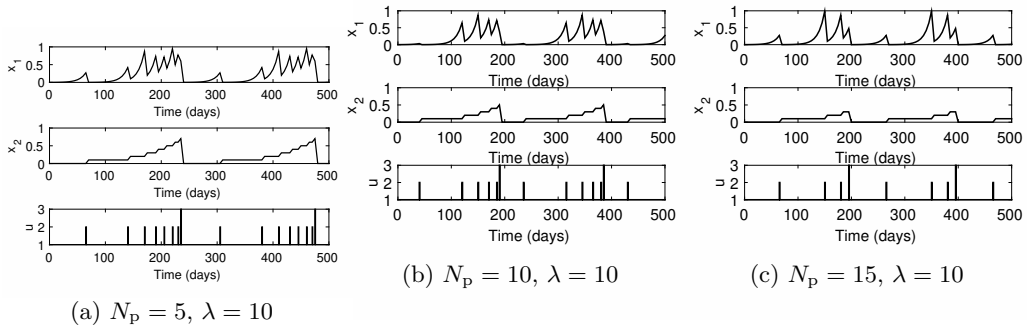
Fig. 5: Predicted state x and control input u for different prediction horizons and a big \lambda
