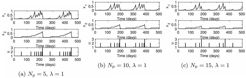
Fig. 4: Predicted state x and control input u for different prediction horizons and a medium \lambda
