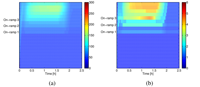
Fig. 9: Mainstream density (9a) and total CO 2 emissions (9b) in the controlled case.
