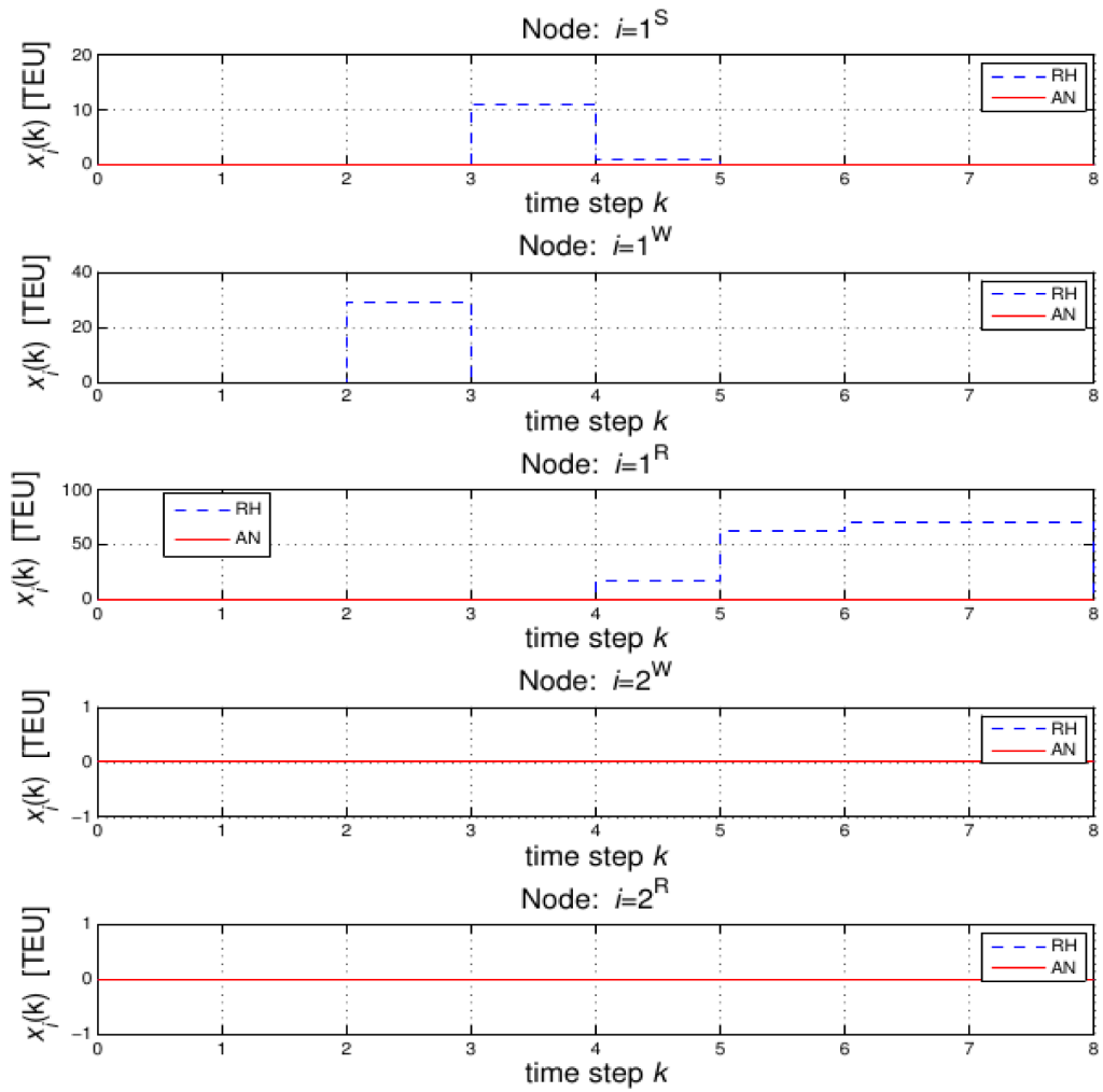
FIGURE 3: The evolution of the number of containers in nodes of the ITN. ‘RH’ and ‘AN’ in the legend denote the receding horizon approach and the all-or-nothing approach, respectively.
