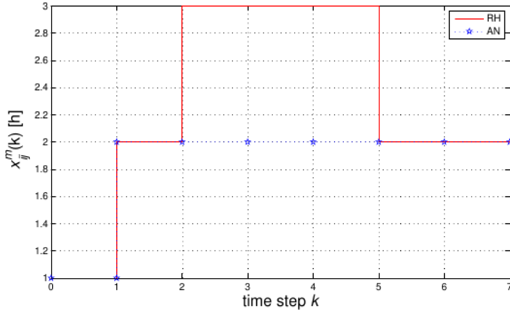
FIGURE 5: The evolution of the link transport time on link 1^R, 2^R . ‘RH’ and ‘AN’ in the legend denote the receding horizon approach and the all-or-nothing approach, respectively.
