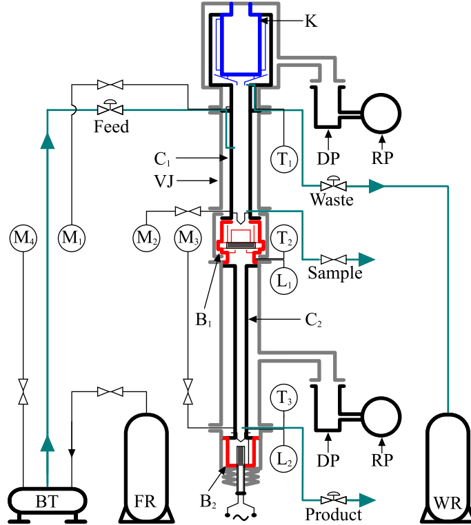
Figure 2: Experimental pilot-scale cryogenic distillation plant with condenser K, primary column C_1 , final column C_2 , reboilers B_1 – B_2 , vacuum jacket VJ, rough pump RP, diffusion pump DP, temperature sensors T_1 – T_3 , manometers M_1 – M_4 , level sensors L_1 – L_2 , feed reservoir FR, buffer tank BT, waste reservoir WR
