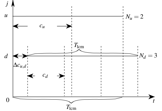
(a) Relationship between cycle times and control time interval
