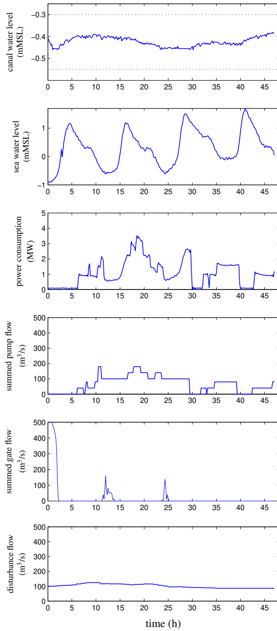
Fig. 1.8: Evolution of the water levels, the flows, and the energy consumption when using MPC.
