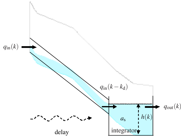
Fig. 1.4: Integrator delay model of a canal reach.
