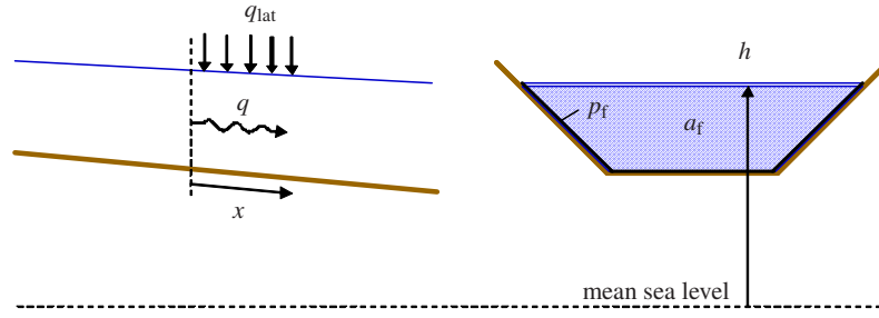
Fig. 1.3: Open-water canal variables and parameters.
