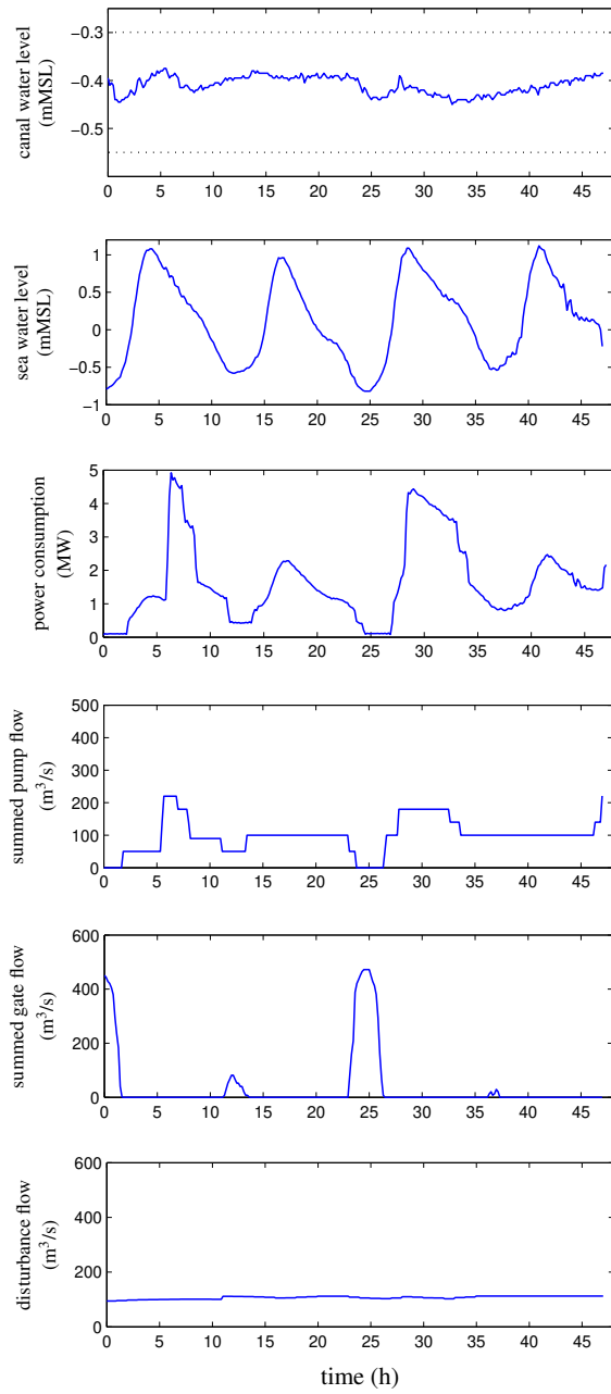
Fig. 1.7: Evolution of the water levels, the flows, and the energy consumption when not using MPC.
