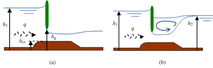
Fig. 1.5: Free-flowing (a) and submerged undershot gate (b).
