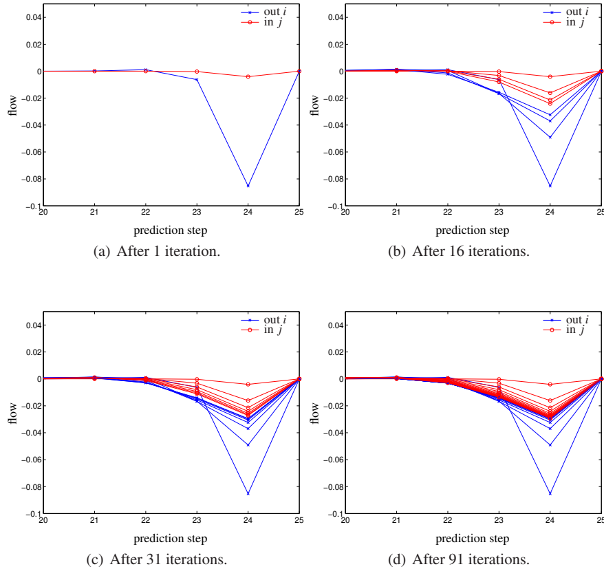
Fig. 1.10: Two MPC controllers obtaining agreement over iterations on how much water should flow between two canal reaches [17].
