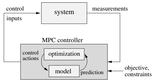
Fig. 2. Illustration of model predictive control.
