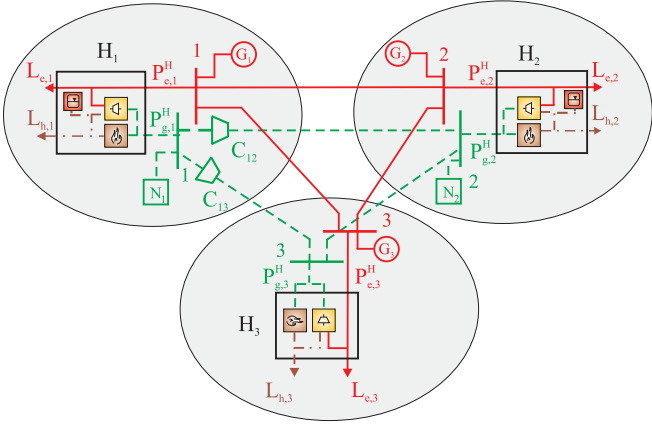
Fig. 1. System setup of three interconnected energy hubs. Active power is provided by generators G_1, G_2, G_3 . Hubs H_1 and H_2 have access to adjacent natural gas networks N_1, N_2 .
