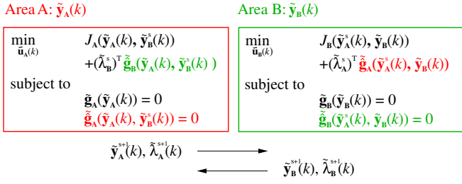
Fig. 3. Decomposition procedure applied to a two-area system (area A: \tilde{\mathbf{y}}_A(k) , area B: \tilde{\mathbf{y}}_B(k) ) and variables to be exchanged after each iteration counter s .
