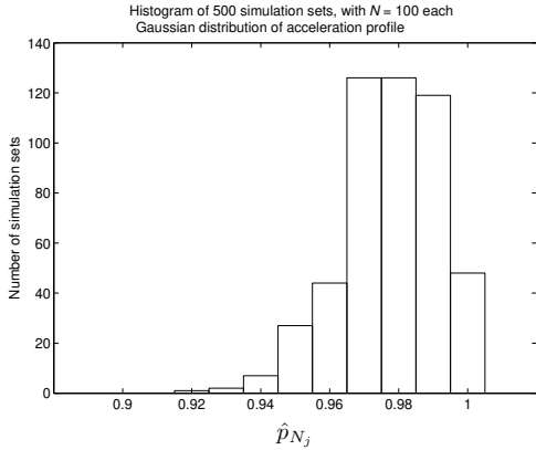
Fig. 3. Histogram of 500 estimates \hat{p}_{N_j} , with N = 100 each, where the acceleration profile is sampled from a Gaussian pdf \mathcal{N}(0, 1.5) .
